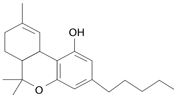
Figure 1: Chemical structure of \Delta^9 -tetrahydrocannabinol.
